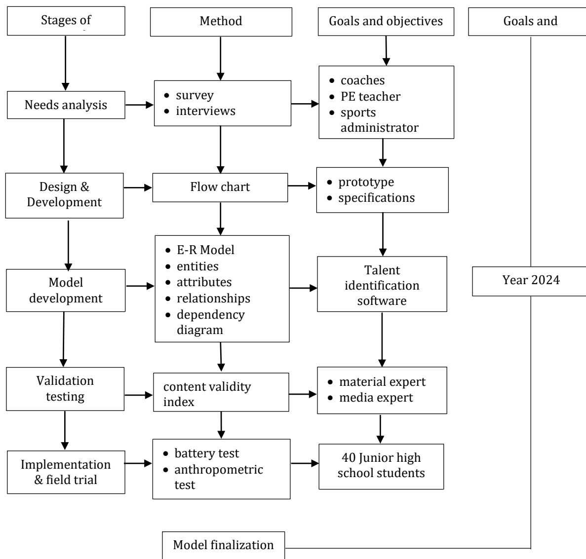
Figure 2. Research Flowchart
